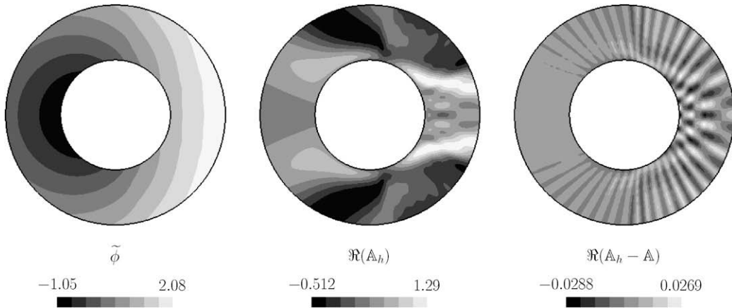
Fig. 8. Neumann problem: approximate phase function \tilde{\phi} and real parts of \mathbb{A}_h and the associated errors. The wave number is k = 25 and the density is n_i = 20 .
