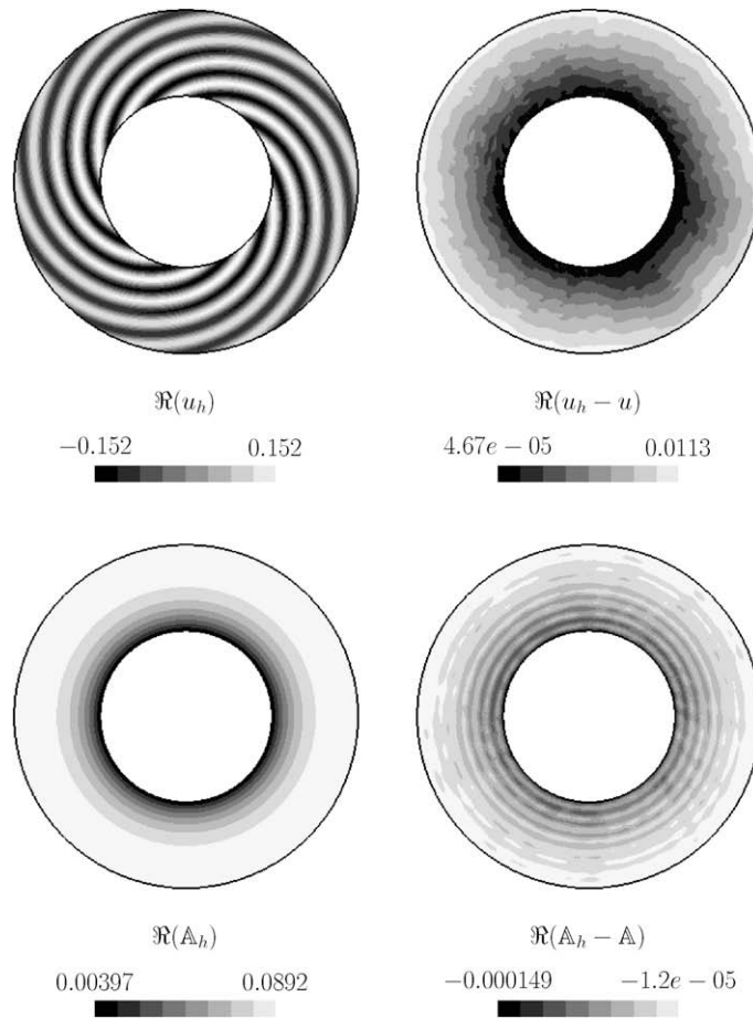
Fig. 4. Neumann problem: real part of u_h and A_h and the associated errors for the mode m = 10 . The wave number is k = 25 and the density is n_\lambda = 20 .
