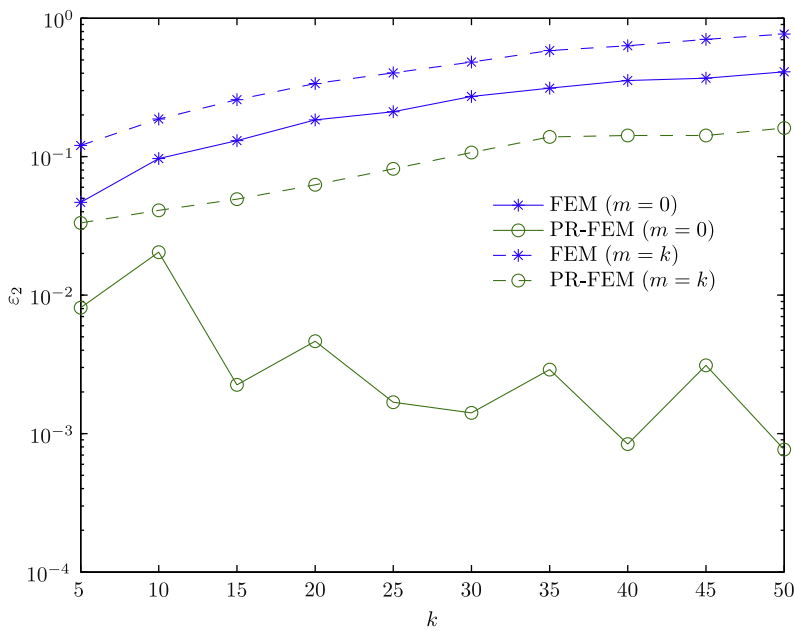
Fig. 6. Neumann problem: evolution of the error \varepsilon_2 for the modes 0 and k with respect to the wave number k , setting n_s = 10 .
