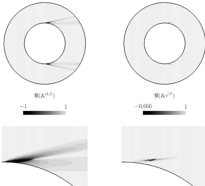
Fig. 22. Choice of the starter: representation of \Re\left(\frac{\Delta^{ik,H}}{|\Delta^{ik,H}|}(\mathbf{x})\right) (left) and \Re\left(\frac{\Delta^{\sqrt{H}}}{|\Delta^{\sqrt{H}}|}(\mathbf{x})\right) (right) for the Neumann problem. We can observe the effect of using the low-order OSRC approximation BC = ik or the high-order model BC = \sqrt{\cdot} . Zooming shows the boundary layer related to the incorporation of creeping waves in the OSRC model. This can affect the PR-FEM since a low-order OSRC would require a local remeshing to the surface for numerically capturing these oscillations.
