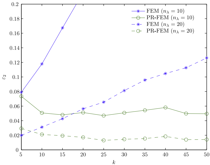
Fig. 9. Neumann problem: evolution of the error \epsilon_2 with respect to the wave number k for two discretizations.
