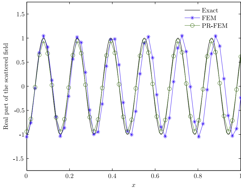
Fig. 1. Real part of the scattered field at a frequency k = 40 for a density of discretization points n_x = 8 . The pollution effect can be observed on the classical FEM approach but is avoided by the PR-FEM formulation.
