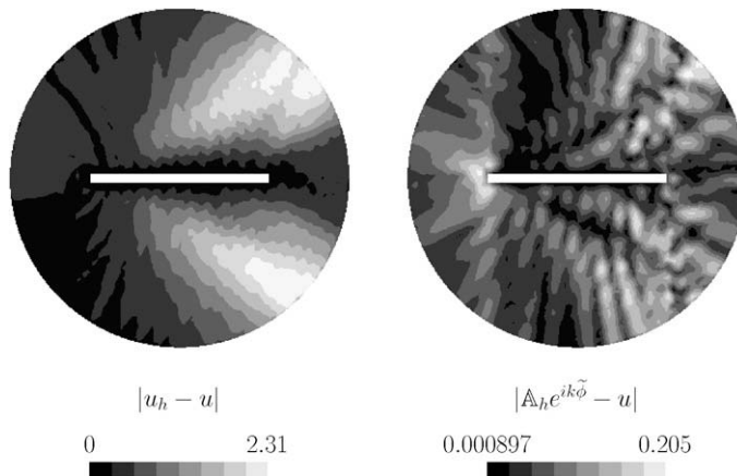
Fig. 18. Dirichlet problem: plate under 45^\circ plane wave incidence for k = 25 and n_z = 4 . Left: absolute error between the reference solution u (computed with n_z = 20 ) and the direct solution u_h . Right: absolute error between the reference solution u and the PR-FEM solution.
