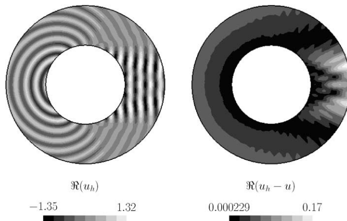
Fig. 7. Neumann problem: real part of u_h and the associated errors. The wave number is k = 25 and the density is n_s = 20 .
