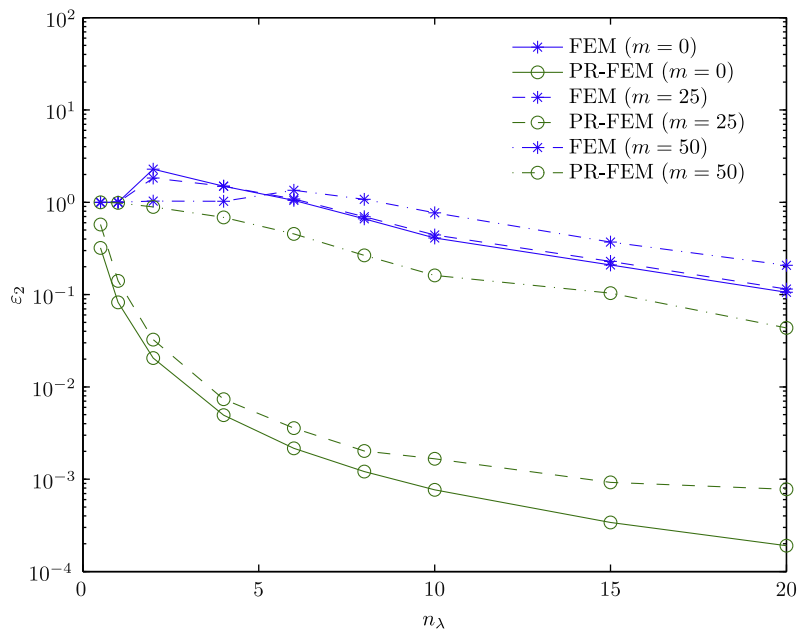
Fig. 5. Neumann problem: evolution of the error e_2 for several modes at k = 50 according to the density of discretization n_\lambda .
